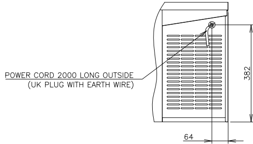
VIEW A (1/10)
